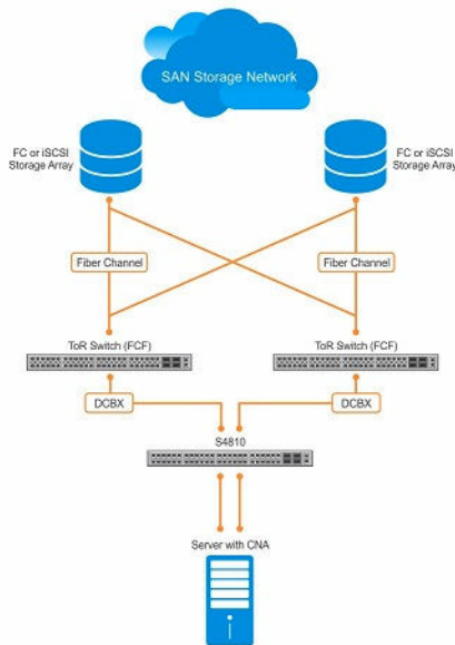
Figure 29. DCBx Sample Topology
